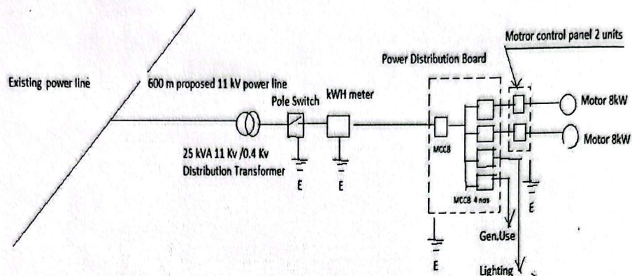
POWER DISTRIBUTION DIAGRAM
